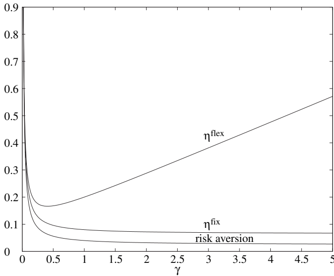
Fig. 1. Precautionary Strength with Cobb-Douglas Utility
